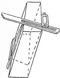
FIG. 279. BEVEL PLACED FOR MITERED HOPPER JOINT.
